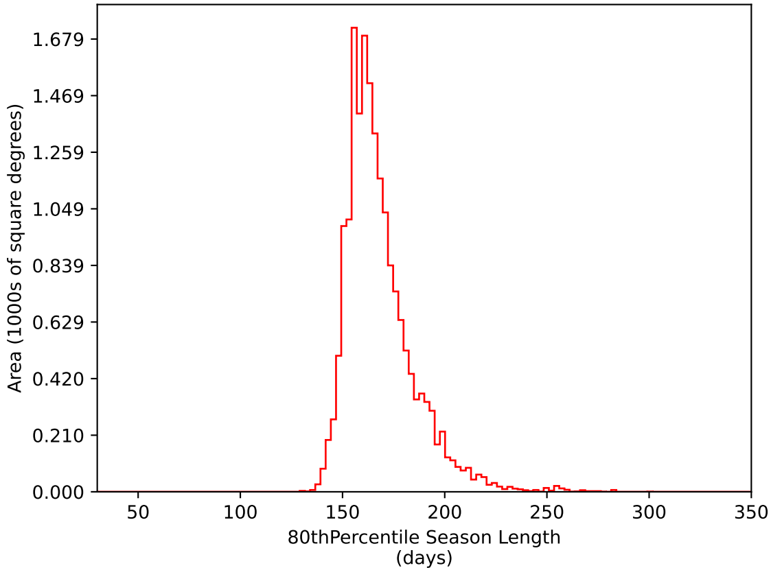
ddf_acor_sf15_lsf20_lsr20_v3.4_10yrs WFD i band: 80thPercentile Season Length
