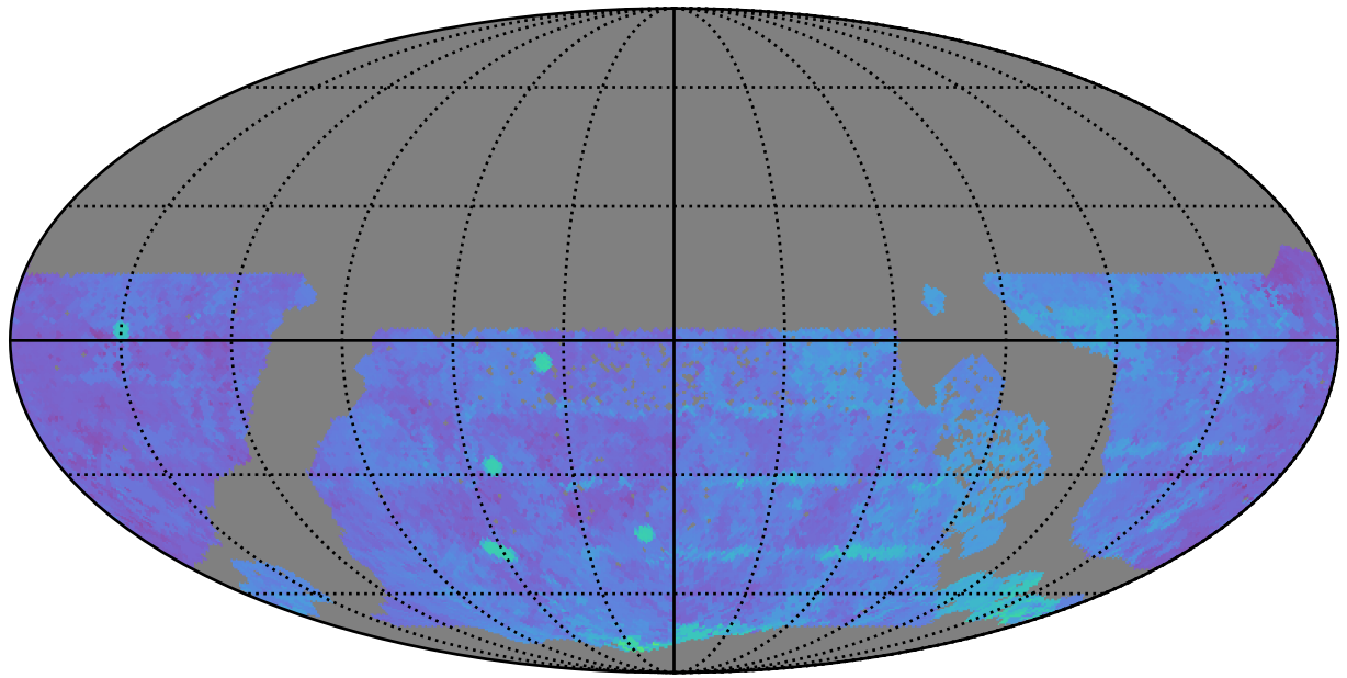
ddf_acor_sf15_lsf20_lsr20_v3.4_10yrs WFD g band: 80thPercentile Season Length
