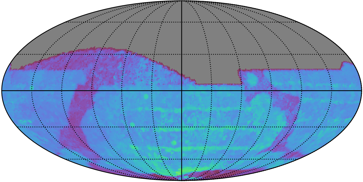
ddf_acor_sf15_lsf20_lsr20_v3.4_10yrs All sky z band: 80thPercentile Season Length
