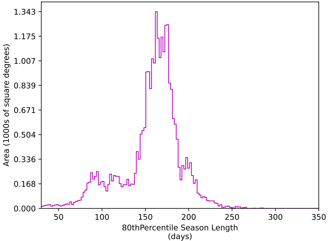
ddf_acor_sf15_lsf20_lsr20_v3.4_10yrs All sky z band: 80thPercentile Season Length
