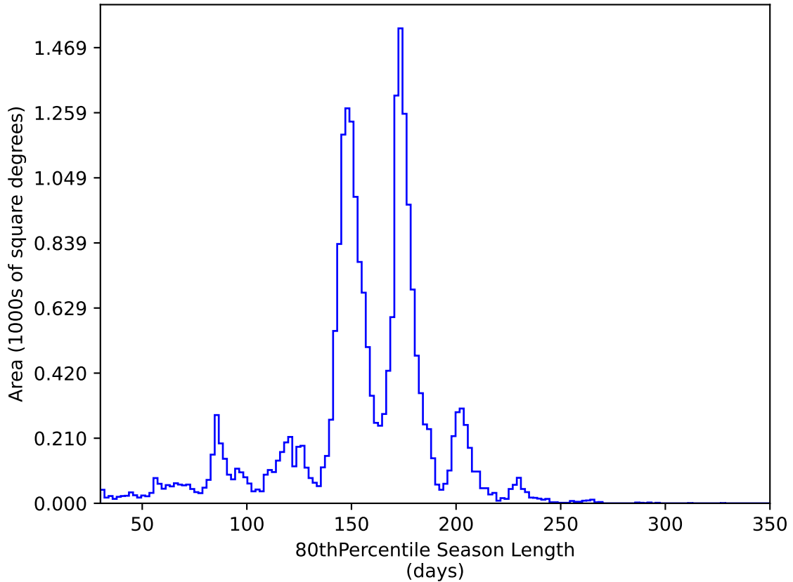
ddf_acor_sf15_lsf20_lsr20_v3.4_10yrs All sky y band: 80thPercentile Season Length
