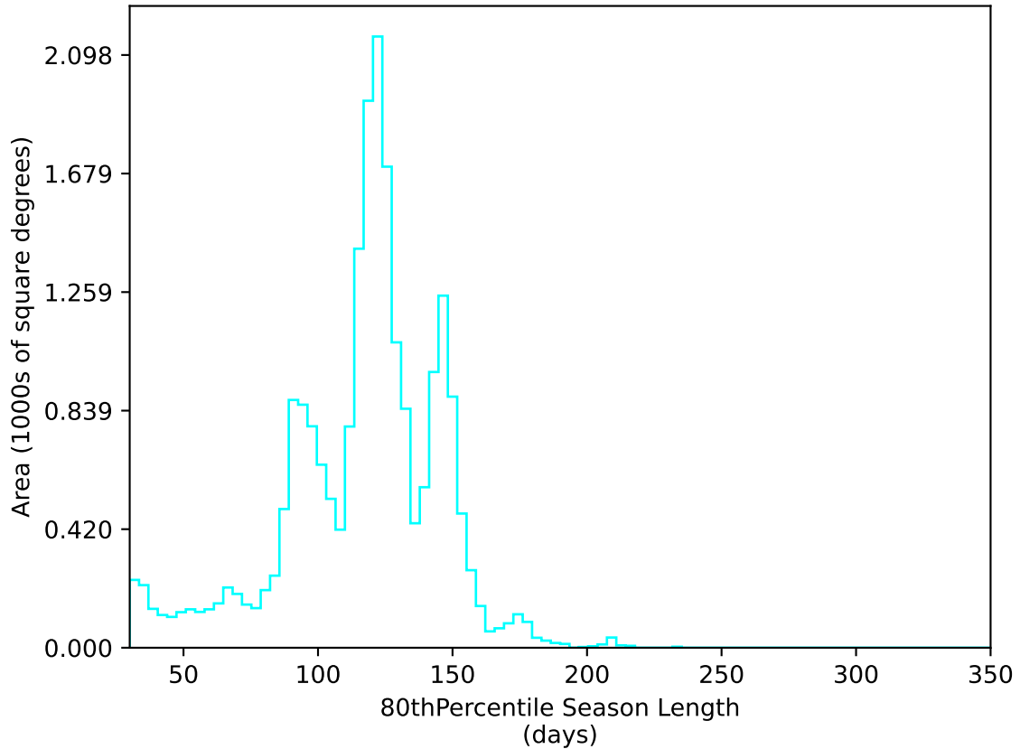
ddf_acor_sf15_lsf20_lsr20_v3.4_10yrs All sky u band: 80thPercentile Season Length
