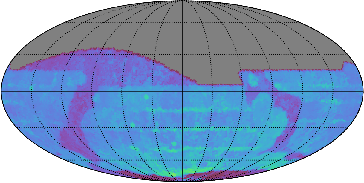
ddf_acor_sf15_lsf20_lsr20_v3.4_10yrs All sky r band: 80thPercentile Season Length
