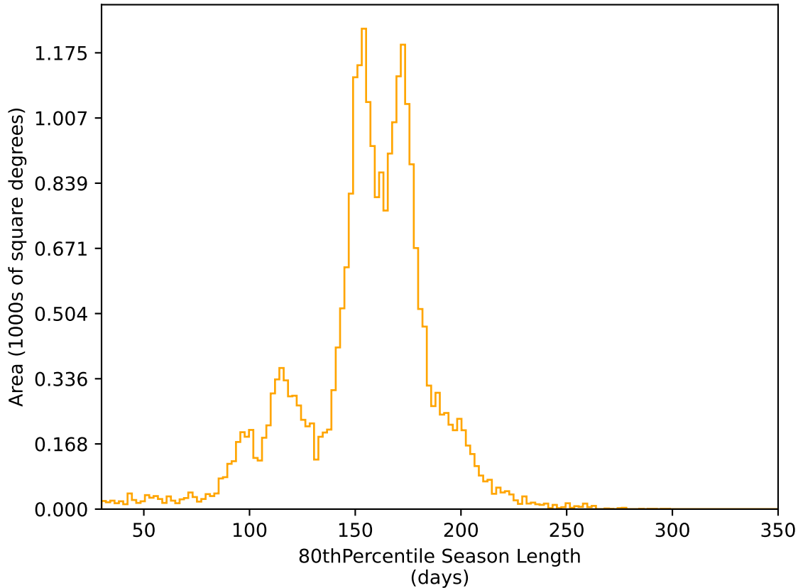
ddf_acor_sf15_lsf20_lsr20_v3.4_10yrs All sky r band: 80thPercentile Season Length
