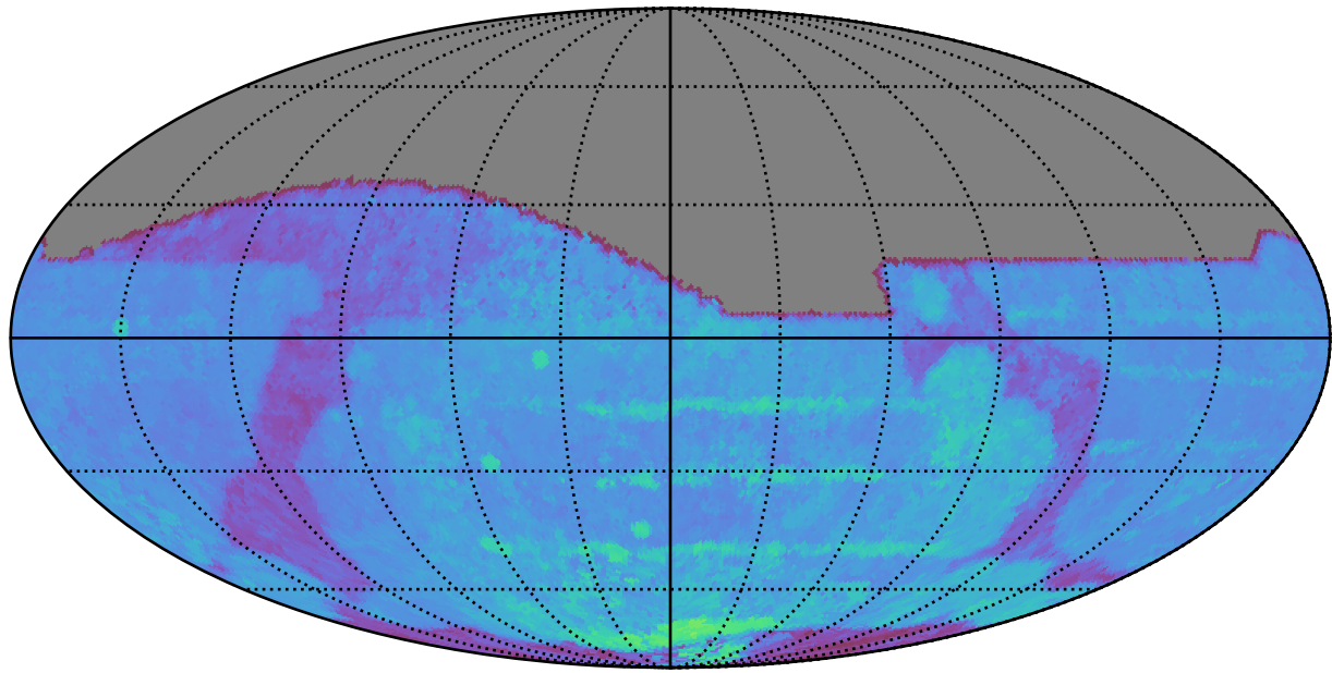
ddf_acor_sf15_lsf20_lsr20_v3.4_10yrs All sky i band: 80thPercentile Season Length
