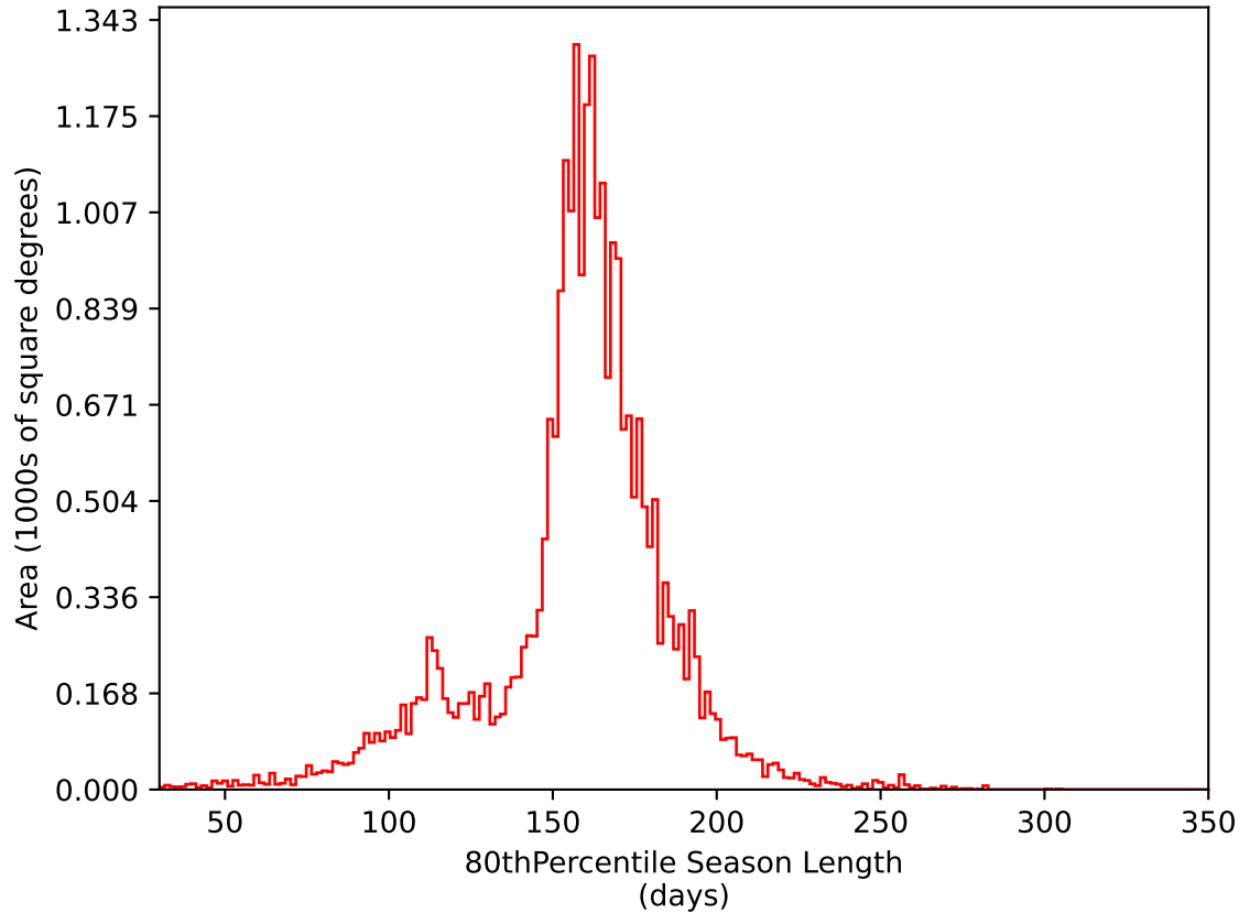
ddf_acor_sf15_lsf20_lsr20_v3.4_10yrs All sky i band: 80thPercentile Season Length
