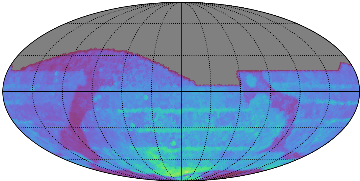
ddf_acor_sf15_lsf20_lsr20_v3.4_10yrs All sky all bands: 80thPercentile Season Length
