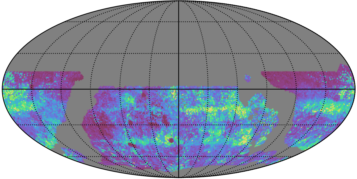
ddf_acor_sf15_lsf20_lsr20_v3.4_10yrs WFD zy bands: 75th Percentile Intranight Timespan
