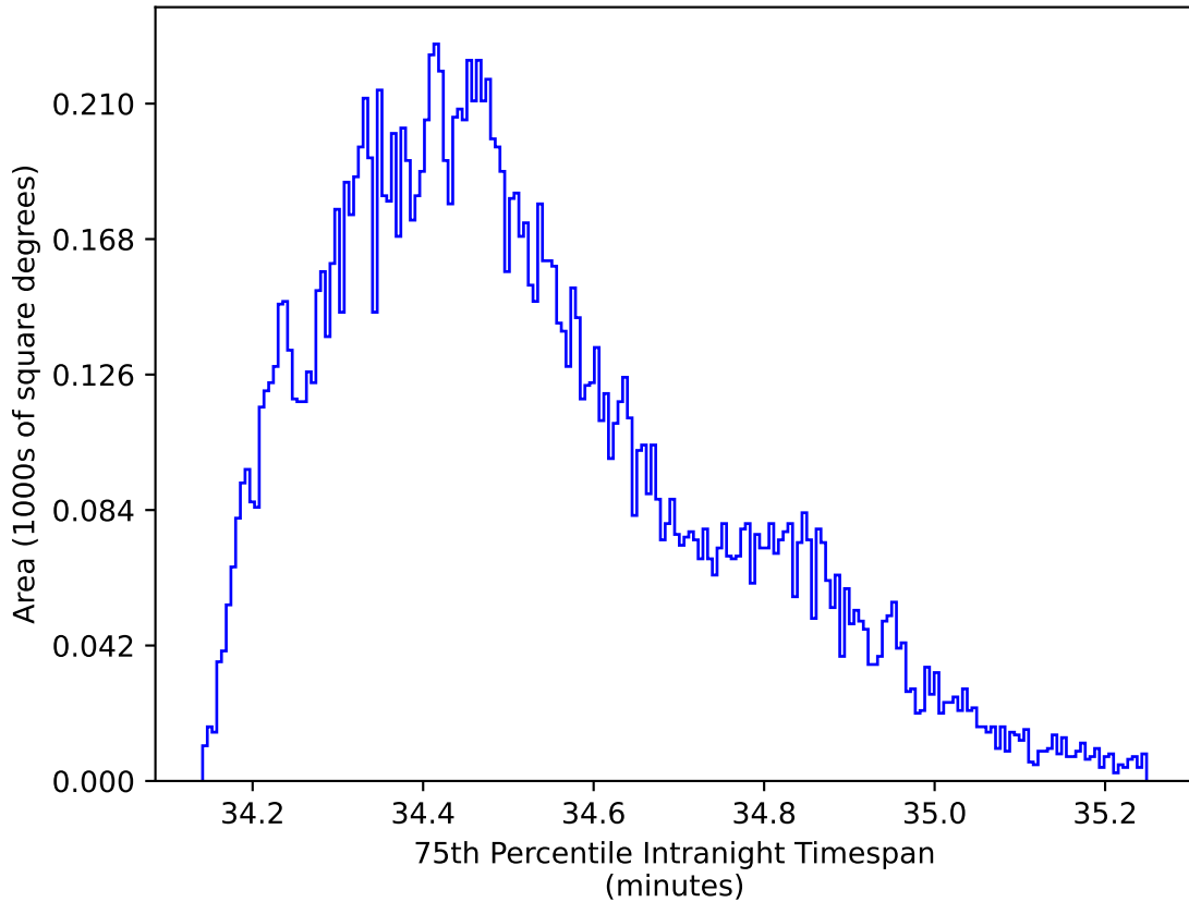
ddf_acor_sf15_lsf20_lsr20_v3.4_10yrs WFD zy bands: 75th Percentile Intranight Timespan
