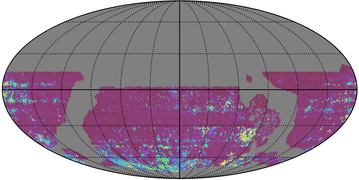
ddf_acor_sf15_lsf20_lsr20_v3.4_10yrs WFD z band: 75th Percentile Intranight Timespan
