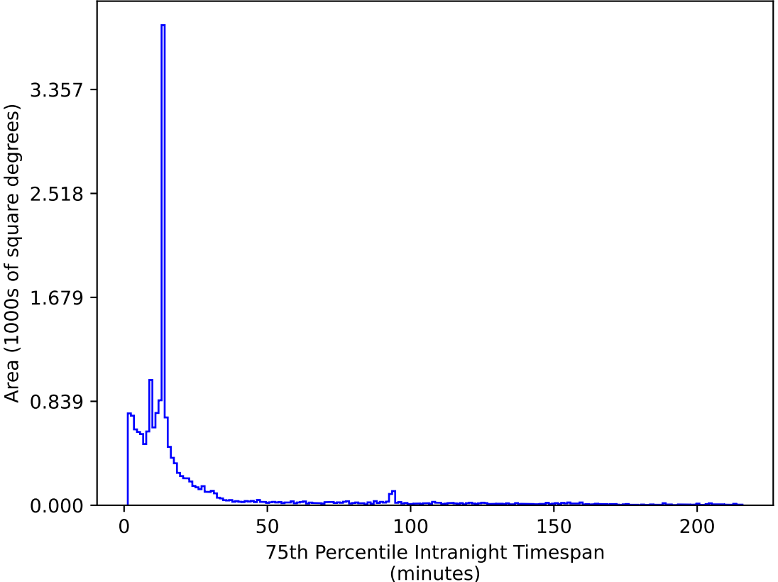
ddf_acor_sf15_lsf20_lsr20_v3.4_10yrs WFD z band: 75th Percentile Intranight Timespan
