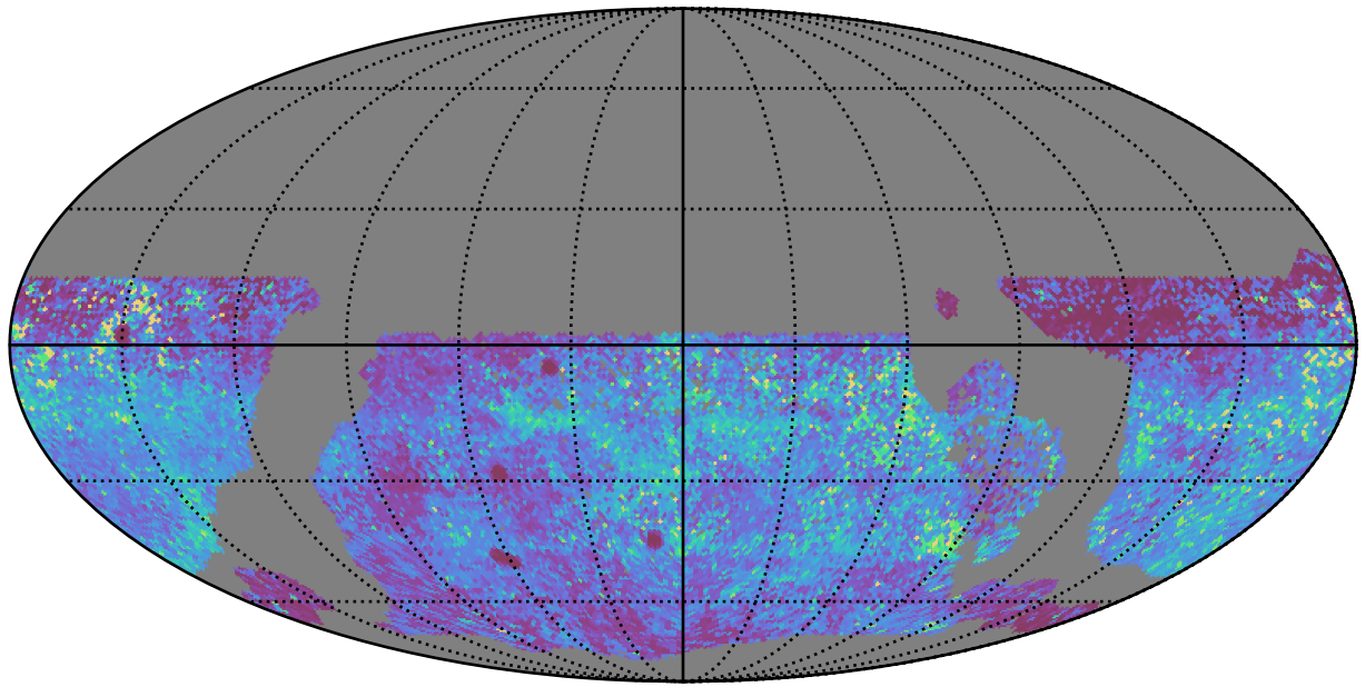
ddf_acor_sf15_lsf20_lsr20_v3.4_10yrs WFD y band: 75th Percentile Intranight Timespan
