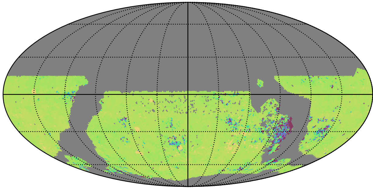
ddf_acor_sf15_lsf20_lsr20_v3.4_10yrs WFD ug bands: 75th Percentile Intranight Timespan
