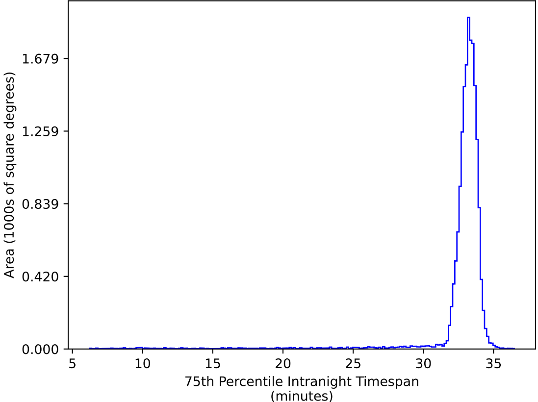
ddf_acor_sf15_lsf20_lsr20_v3.4_10yrs WFD ug bands: 75th Percentile Intranight Timespan
