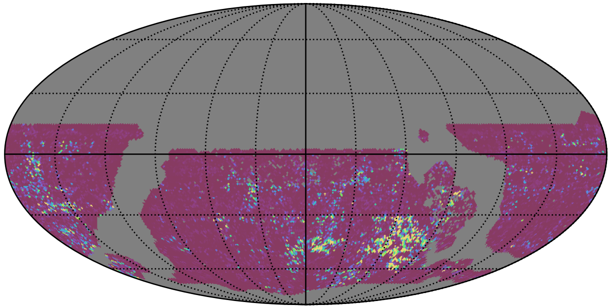
ddf_acor_sf15_lsf20_lsr20_v3.4_10yrs WFD u band: 75th Percentile Intranight Timespan
