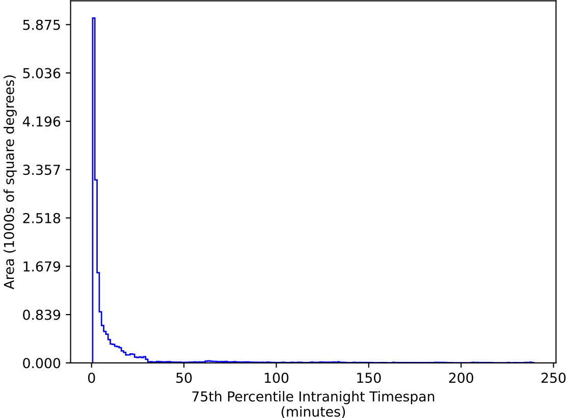
ddf_acor_sf15_lsf20_lsr20_v3.4_10yrs WFD u band: 75th Percentile Intranight Timespan
