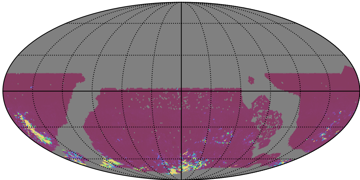
ddf_acor_sf15_lsf20_lsr20_v3.4_10yrs WFD ri bands: 75th Percentile Intranight Timespan
