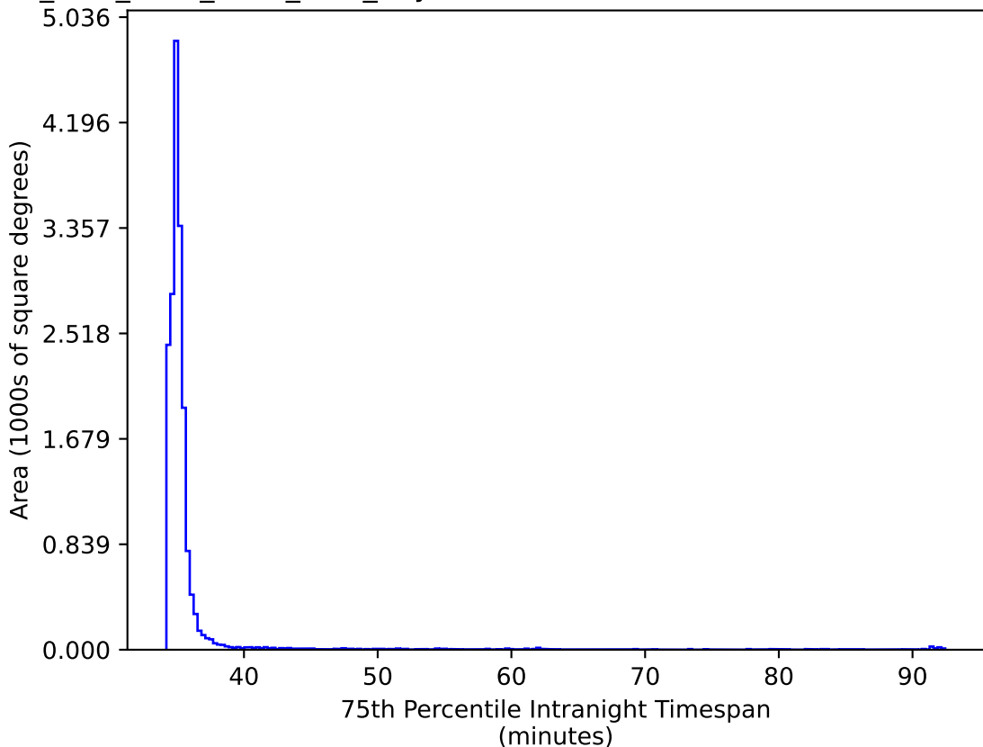
ddf_acor_sf15_lsf20_lsr20_v3.4_10yrs WFD ri bands: 75th Percentile Intranight Timespan
