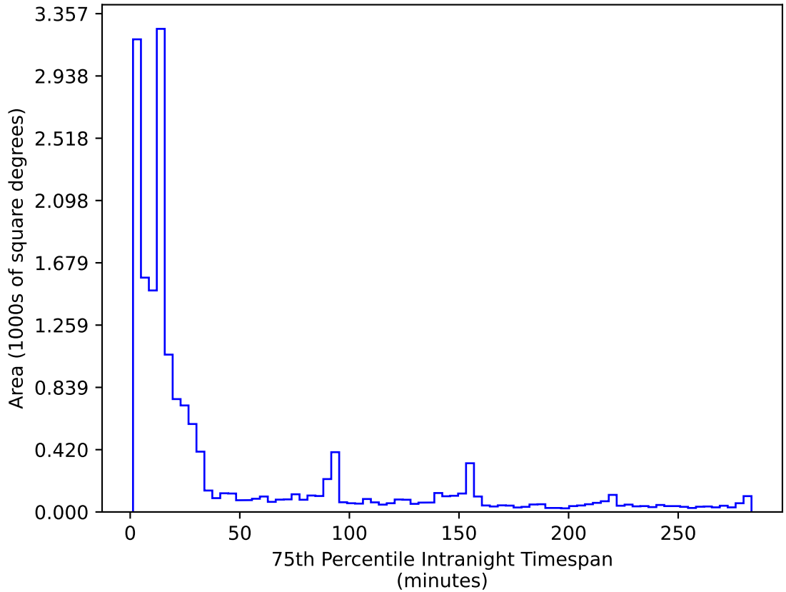
ddf_acor_sf15_lsf20_lsr20_v3.4_10yrs WFD r band: 75th Percentile Intranight Timespan
