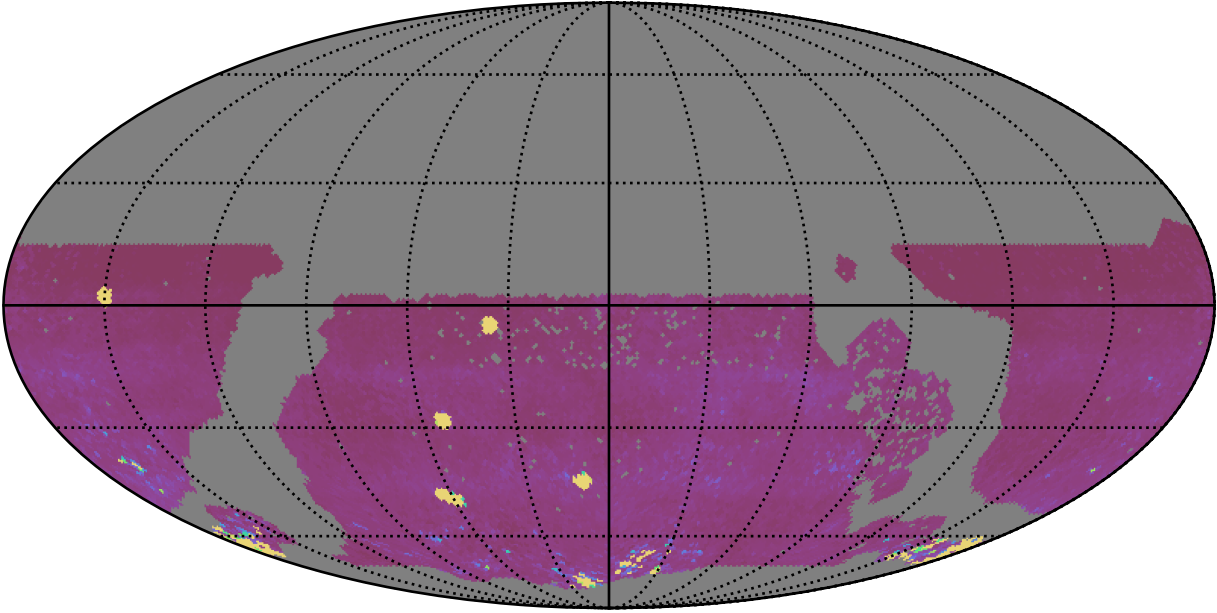
ddf_acor_sf15_lsf20_lsr20_v3.4_10yrs WFD iz bands: 75th Percentile Intranight Timespan
