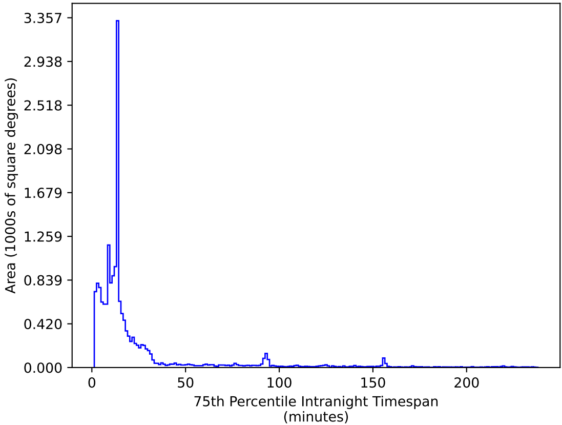
ddf_acor_sf15_lsf20_lsr20_v3.4_10yrs WFD i band: 75th Percentile Intranight Timespan
