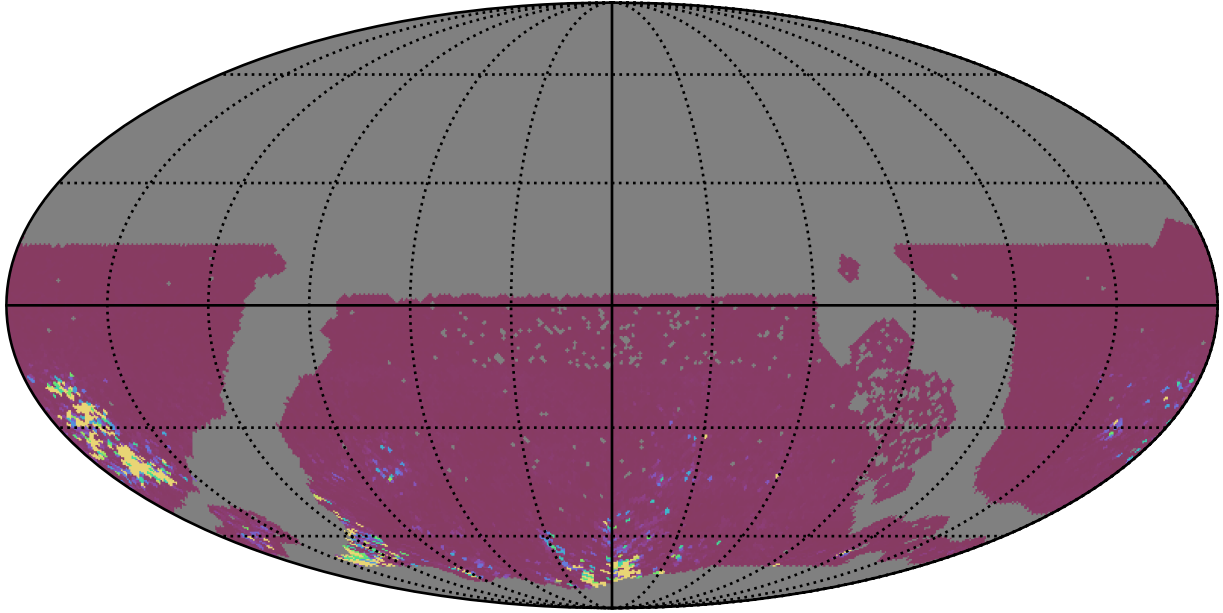
ddf_acor_sf15_lsf20_lsr20_v3.4_10yrs WFD gr bands: 75th Percentile Intranight Timespan
