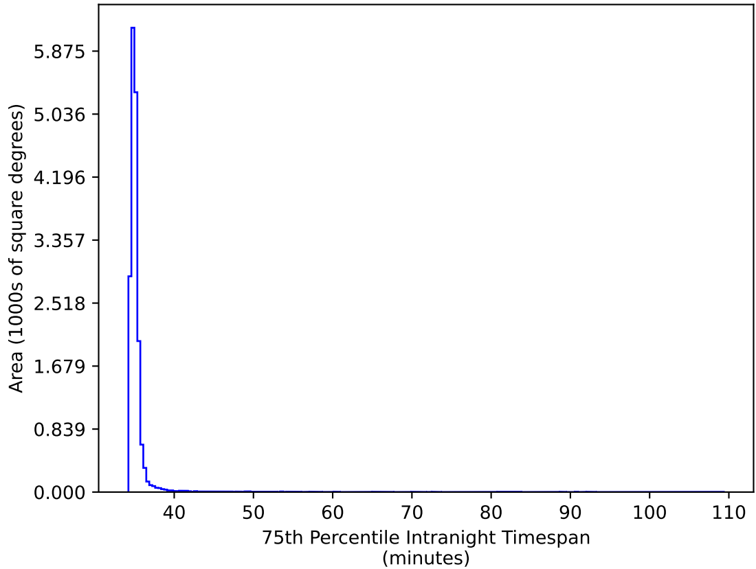
ddf_acor_sf15_lsf20_lsr20_v3.4_10yrs WFD gr bands: 75th Percentile Intranight Timespan
