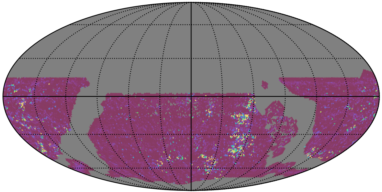
ddf_acor_sf15_lsf20_lsr20_v3.4_10yrs WFD g band: 75th Percentile Intranight Timespan
