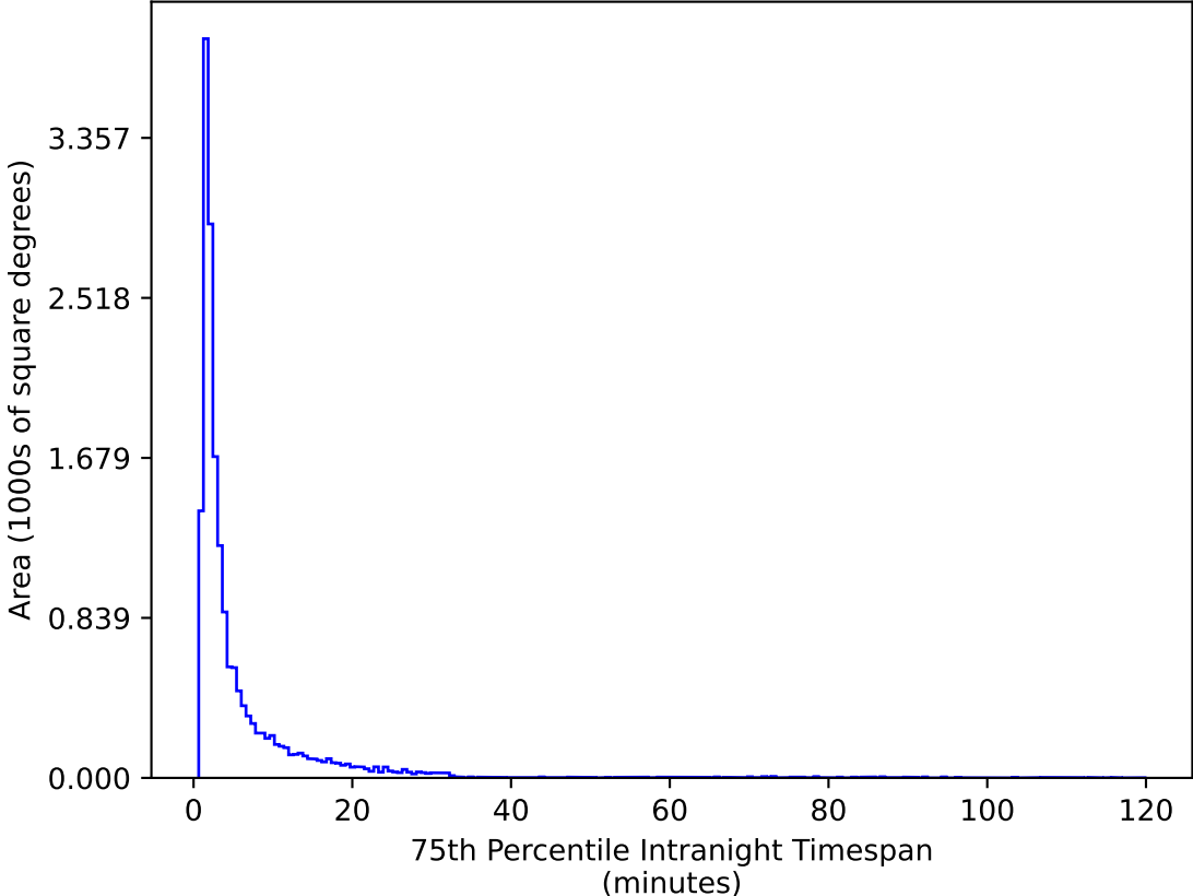
ddf_acor_sf15_lsf20_lsr20_v3.4_10yrs WFD g band: 75th Percentile Intranight Timespan
