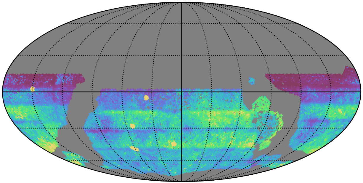
ddf_acor_sf15_lsf20_lsr20_v3.4_10yrs WFD all bands: 75th Percentile Intranight Timespan
