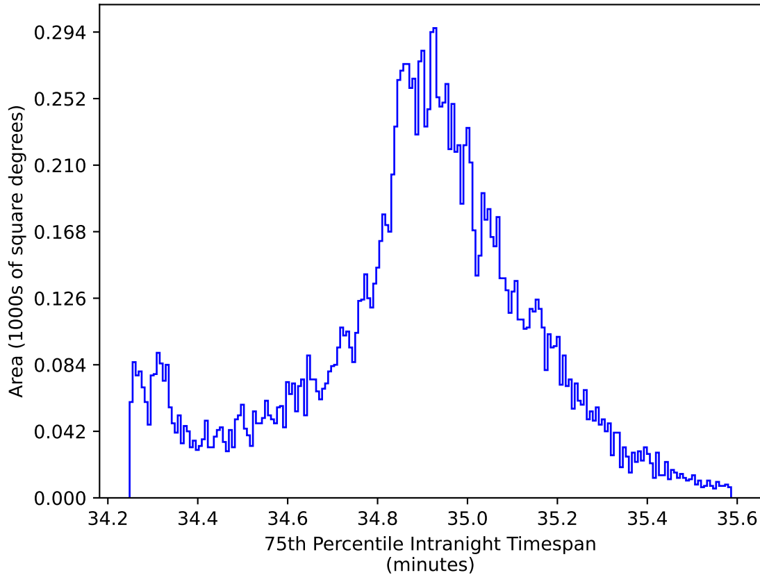
ddf_acor_sf15_lsf20_lsr20_v3.4_10yrs WFD all bands: 75th Percentile Intranight Timespan
