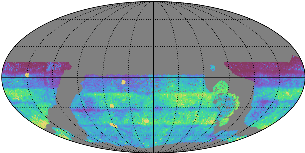
ddf_acor_sf15_lsf20_lsr20_v3.4_10yrs WFD: 75th Percentile Intranight Timespan
