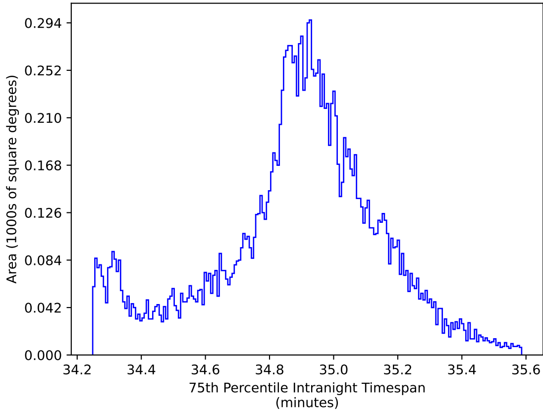
ddf_acor_sf15_lsf20_lsr20_v3.4_10yrs WFD: 75th Percentile Intranight Timespan
