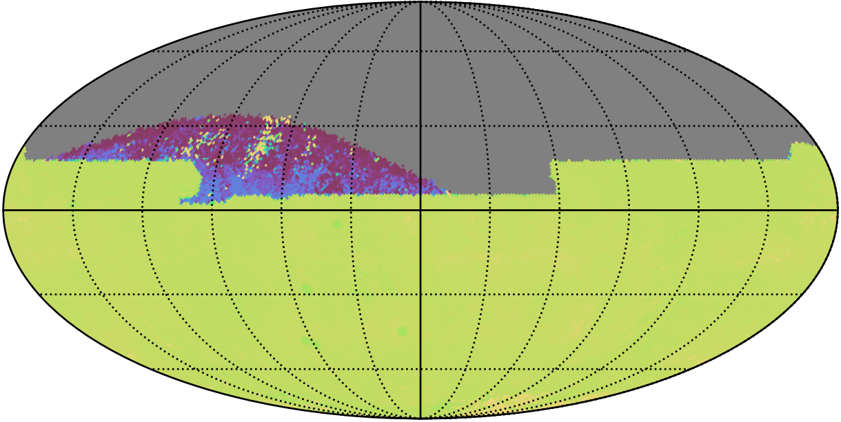
ddf_acor_sf15_lsf20_lsr20_v3.4_10yrs All sky zy bands: 75th Percentile Intranight Timespan
