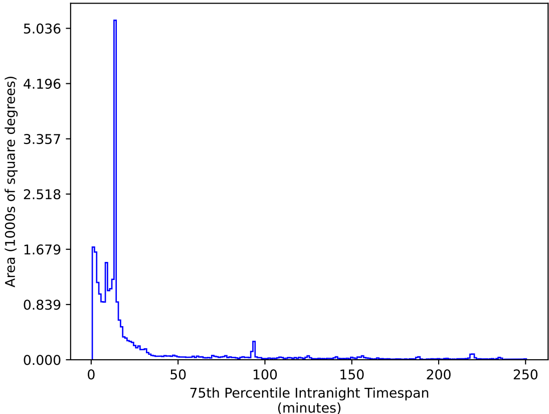
ddf_acor_sf15_lsf20_lsr20_v3.4_10yrs All sky z band: 75th Percentile Intranight Timespan
