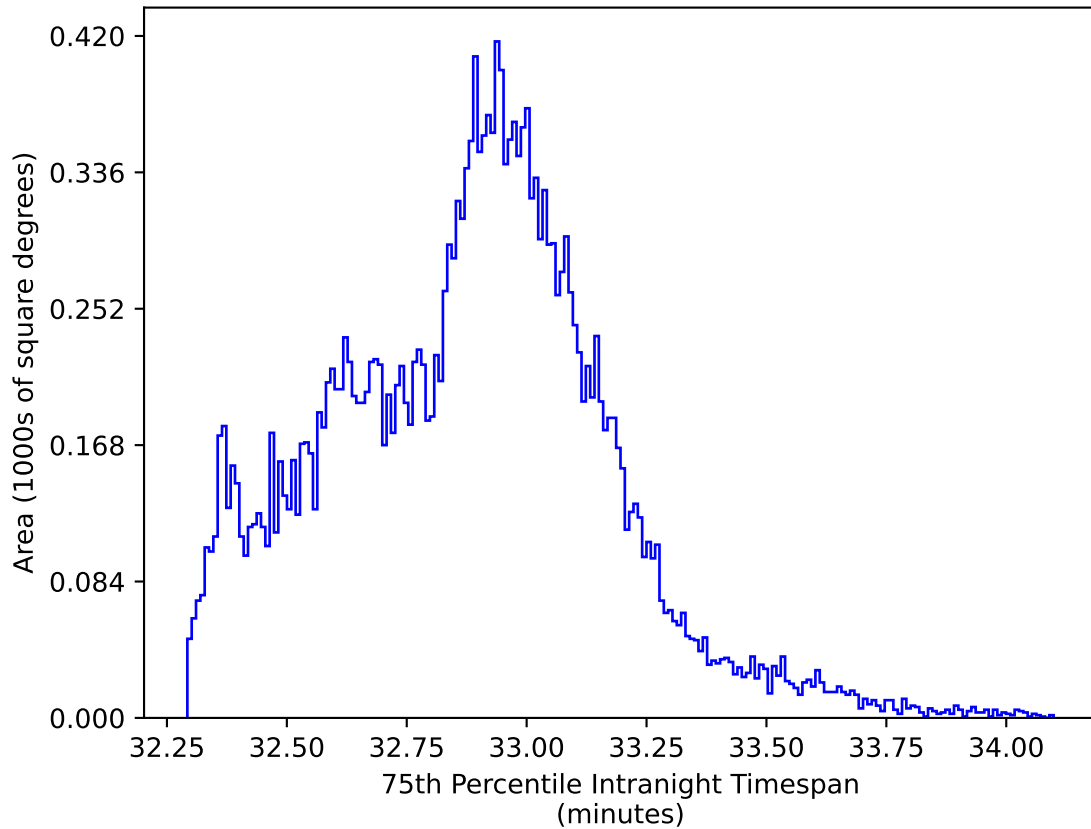
ddf_acor_sf15_lsf20_lsr20_v3.4_10yrs All sky y band: 75th Percentile Intranight Timespan
