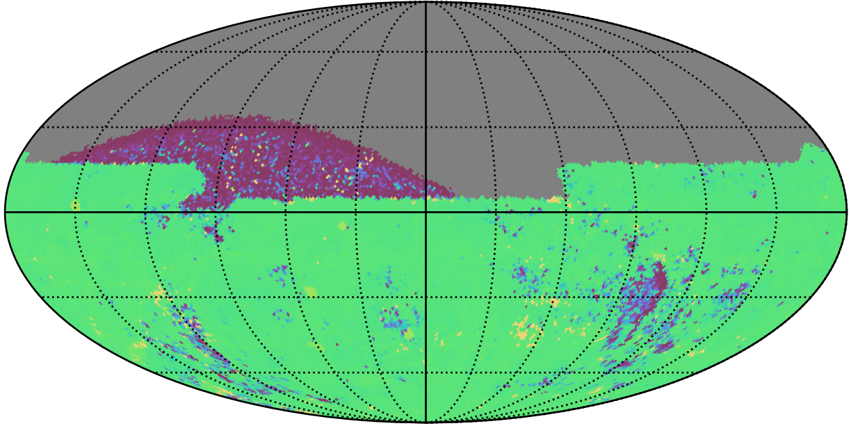
ddf_acor_sf15_lsf20_lsr20_v3.4_10yrs All sky ug bands: 75th Percentile Intranight Timespan
