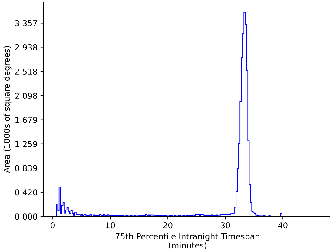
ddf_acor_sf15_lsf20_lsr20_v3.4_10yrs All sky ug bands: 75th Percentile Intranight Timespan
