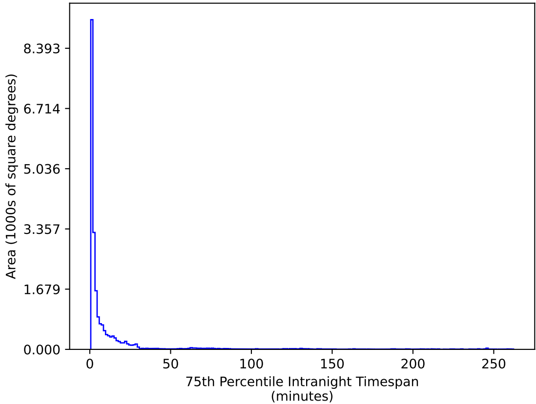
ddf_acor_sf15_lsf20_lsr20_v3.4_10yrs All sky u band: 75th Percentile Intranight Timespan
