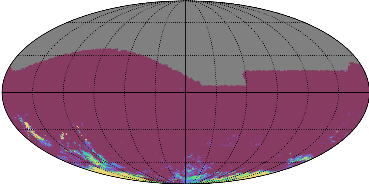
ddf_acor_sf15_lsf20_lsr20_v3.4_10yrs All sky ri bands: 75th Percentile Intranight Timespan
