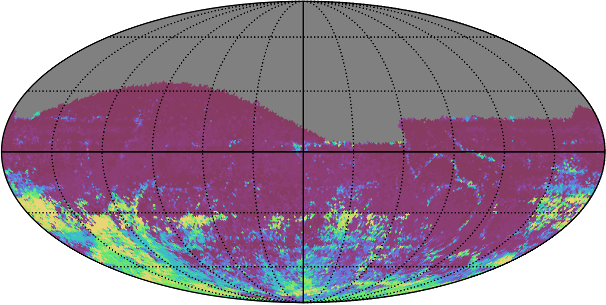
ddf_acor_sf15_lsf20_lsr20_v3.4_10yrs All sky r band: 75th Percentile Intranight Timespan
