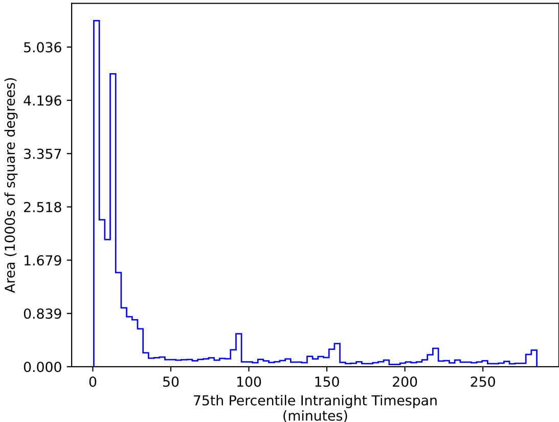
ddf_acor_sf15_lsf20_lsr20_v3.4_10yrs All sky r band: 75th Percentile Intranight Timespan
