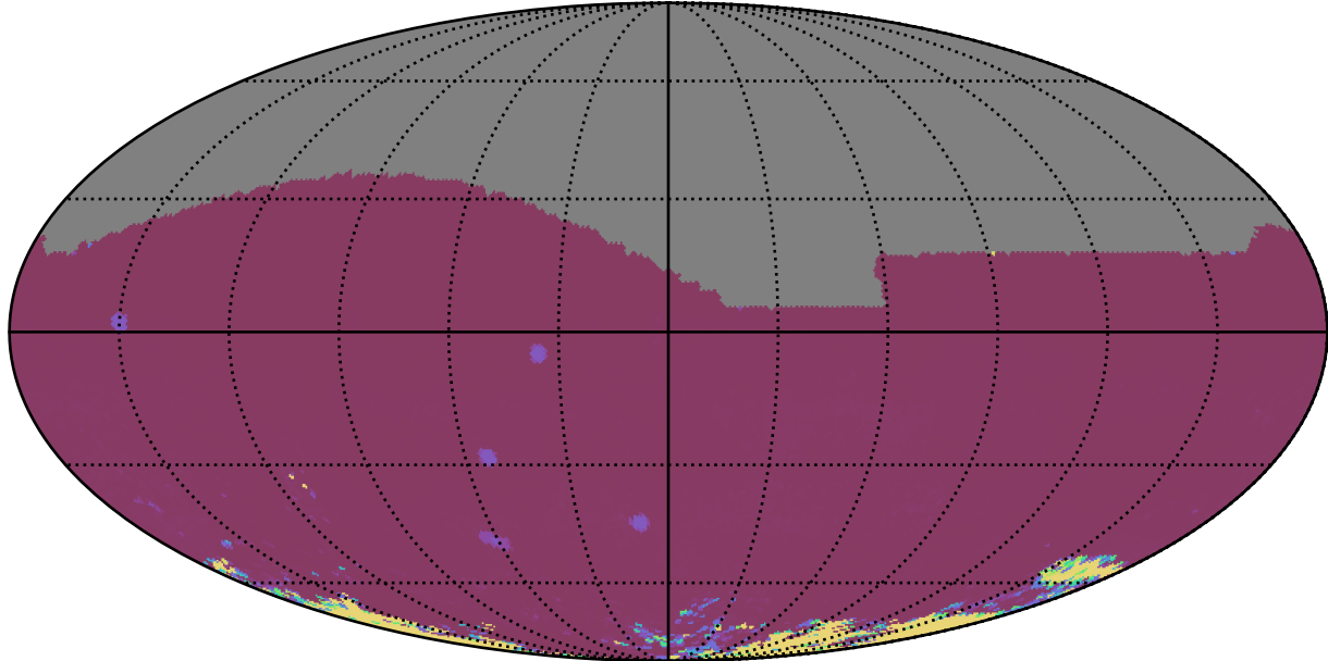
ddf_acor_sf15_lsf20_lsr20_v3.4_10yrs All sky iz bands: 75th Percentile Intranight Timespan
