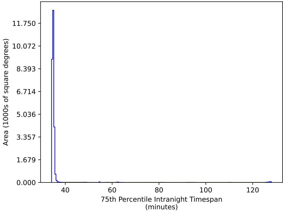
ddf_acor_sf15_lsf20_lsr20_v3.4_10yrs All sky iz bands: 75th Percentile Intranight Timespan
