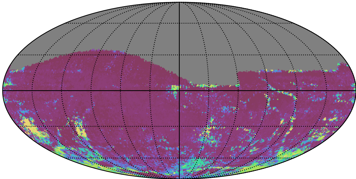
ddf_acor_sf15_lsf20_lsr20_v3.4_10yrs All sky i band: 75th Percentile Intranight Timespan
