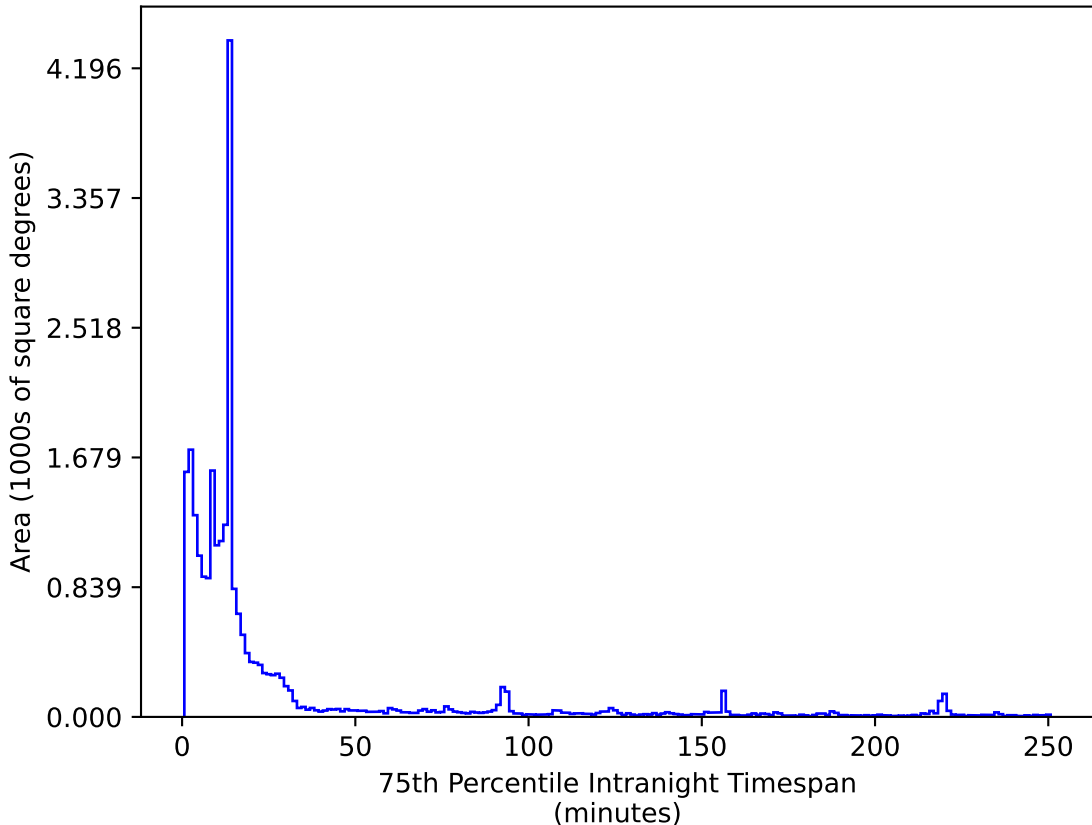
ddf_acor_sf15_lsf20_lsr20_v3.4_10yrs All sky i band: 75th Percentile Intranight Timespan
