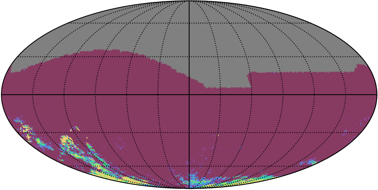
ddf_acor_sf15_lsf20_lsr20_v3.4_10yrs All sky gr bands: 75th Percentile Intranight Timespan
