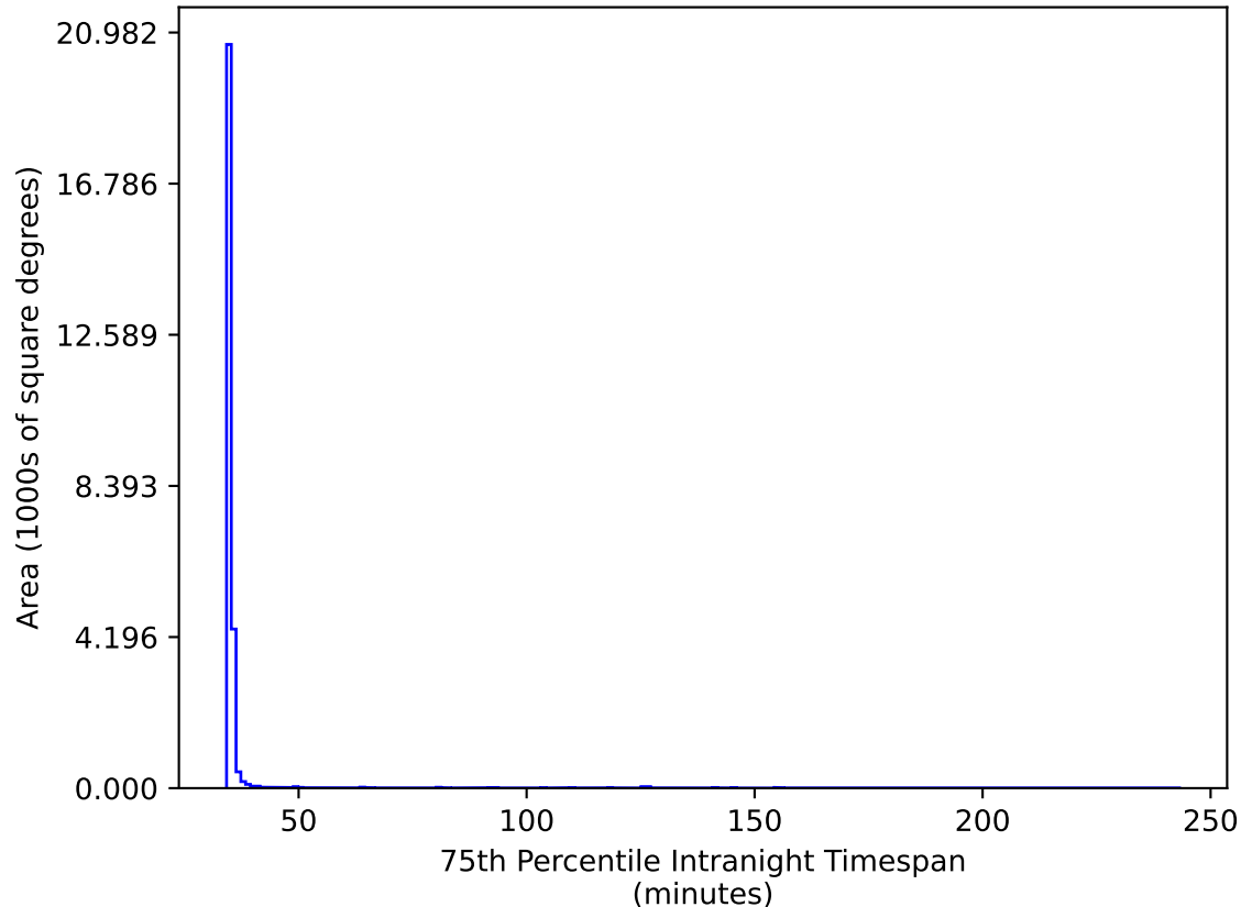
ddf_acor_sf15_lsf20_lsr20_v3.4_10yrs All sky gr bands: 75th Percentile Intranight Timespan
