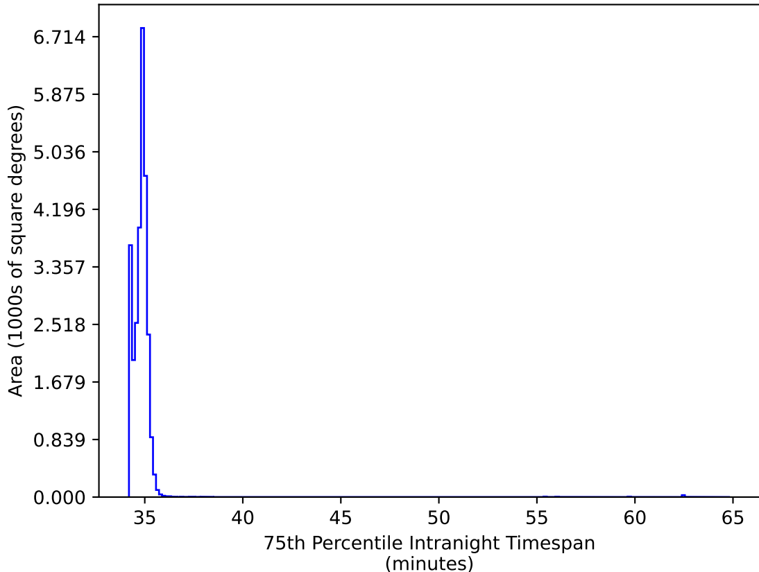
ddf_acor_sf15_lsf20_lsr20_v3.4_10yrs All sky all bands: 75th Percentile Intranight Timespan
