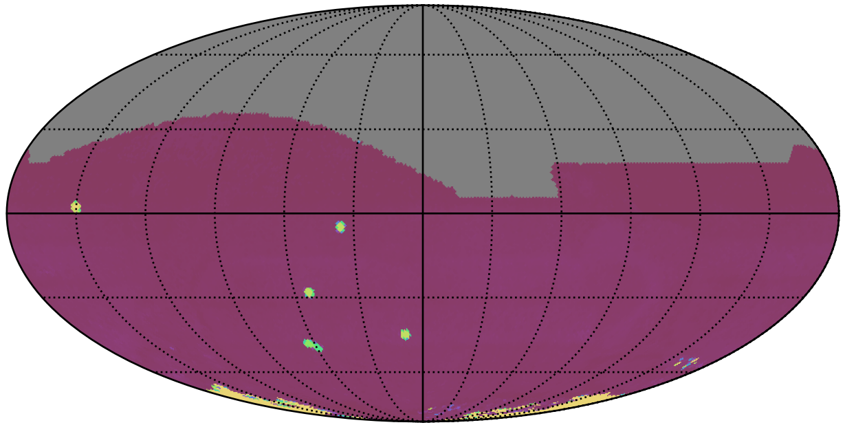
ddf_acor_sf15_lsf20_lsr20_v3.4_10yrs All sky: 75th Percentile Intranight Timespan
